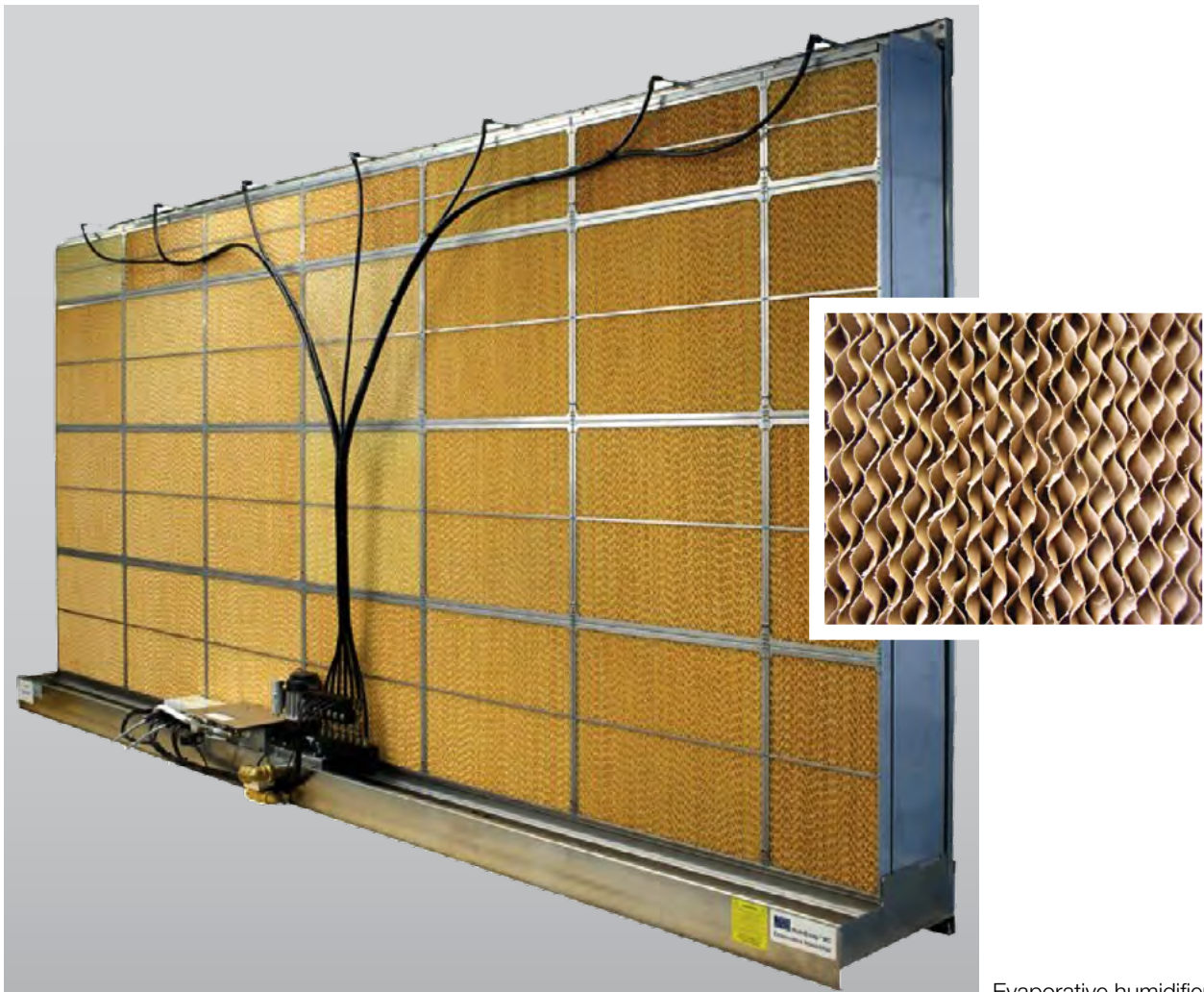
Evaporative humidifier
