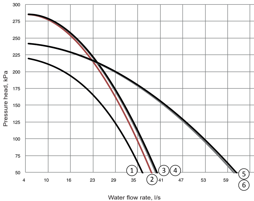
High-pressure variable-speed dual pump (Hydraulic module option 116W)
