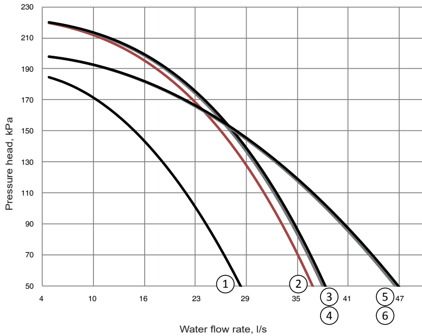
Low-pressure variable-speed dual pump (Hydraulic module option 116A)
